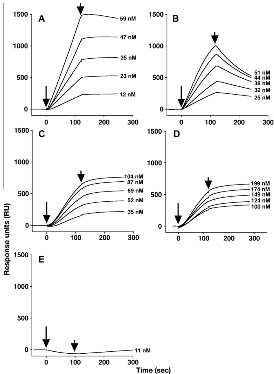
Fig. 2. Binding of various growth factors to the immobilized shrimp HS. Various concentrations of FGF-2 (A), FGF-1 (B), PTN (C), or MK (D) were injected onto the surface of a shrimp HS-immobilized sensor chip. Sensorgrams were overlaid using the BIA evaluation software (version 4. 1). Concentrations of each growth factor are shown on the right. Long and short arrows indicate the beginning of the association and dissociation phases, respectively. No significant binding of HGF at 11 nM was detected (E).
